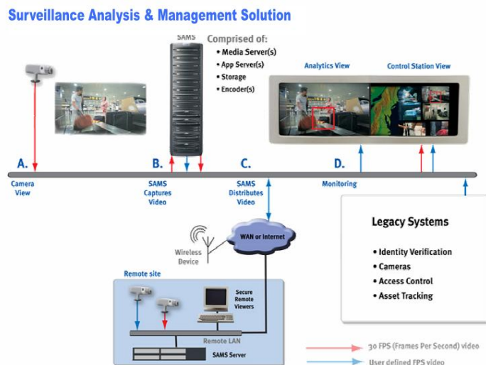
In the diagram, the Surveillance Analysis and Management Solution consists of video server software on an industry-standard Linux server, EMC storage platforms (SAN, NAS or CAS) and related storage management software, together with Verizon Business/EMC infrastructure assessment and integration services.
